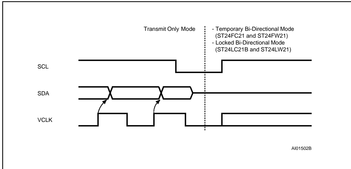
Figure 4. Transition Mode Waveforms
