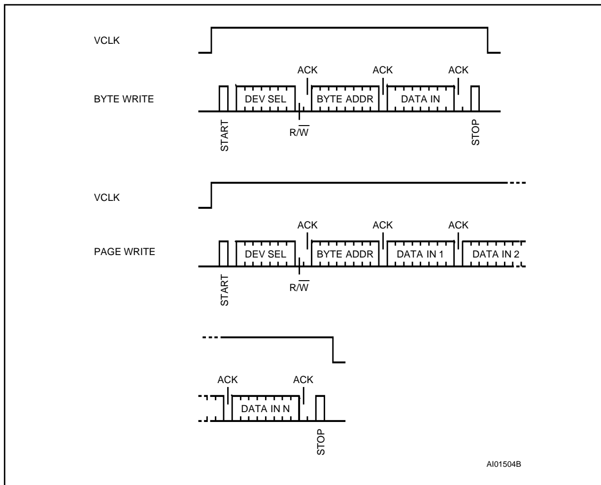
Figure 11. Write Modes Sequence
